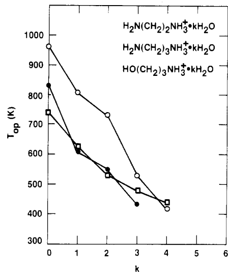
Figure 1. The effects of external hydration on the stability of intramolecular hydrogen bonds in \text{NH}_2(\text{CH}_2)_3\text{NH}_3^+ \cdot k\text{H}_2\text{O} (O), \text{NH}_2(\text{CH}_2)_2\text{NH}_3^+ \cdot k\text{H}_2\text{O} (●), and \text{HO}(\text{CH}_2)_3\text{NH}_3^+ \cdot k\text{H}_2\text{O} (□).
