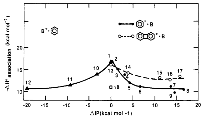
Figure 2. \Delta H^\circ_{D^{\cdot-}} of radical dimer ions as a function of the difference between the ionization potentials of the components ( \Delta IP ), in three sets of dimers. Set I (●): benzene + ·B, where B is (1) benzene, (2) 2-fluoro-, (3) 1,2-difluoro-, (4) 1,3-difluoro-, (5) 1,2,4,5-tetrafluoro-, (6) 1,2,3,5-tetrafluoro-, (7) pentafluoro-, (8) hexafluorobenzene, (9) cyclohexane. Set II (▲): B + ·benzene, where B + is (10) chlorobenzene + , (11) toluene + , (12) 1,3,5-trimethylbenzene + . Set III (○): Biphenylene + ·B, where B is (13) biphenylene, (14) acenaphthylene, (15) benzoindene, (16) naphthalene, (17) biphenylene and (18) (□) represents the benzene H + -benzene dimer. Note that the difference between the maximum and the asymptotic limit is 6 kcal mol -1 in the benzene series but only 3 \pm 1 kcal mol -1 in the biphenylene series, which indicates \Delta H^\circ_{\text{resonance}} = 6 kcal mol -1 in benzene 2 + but only 3 kcal mol -1 in biphenylene 2 + .
